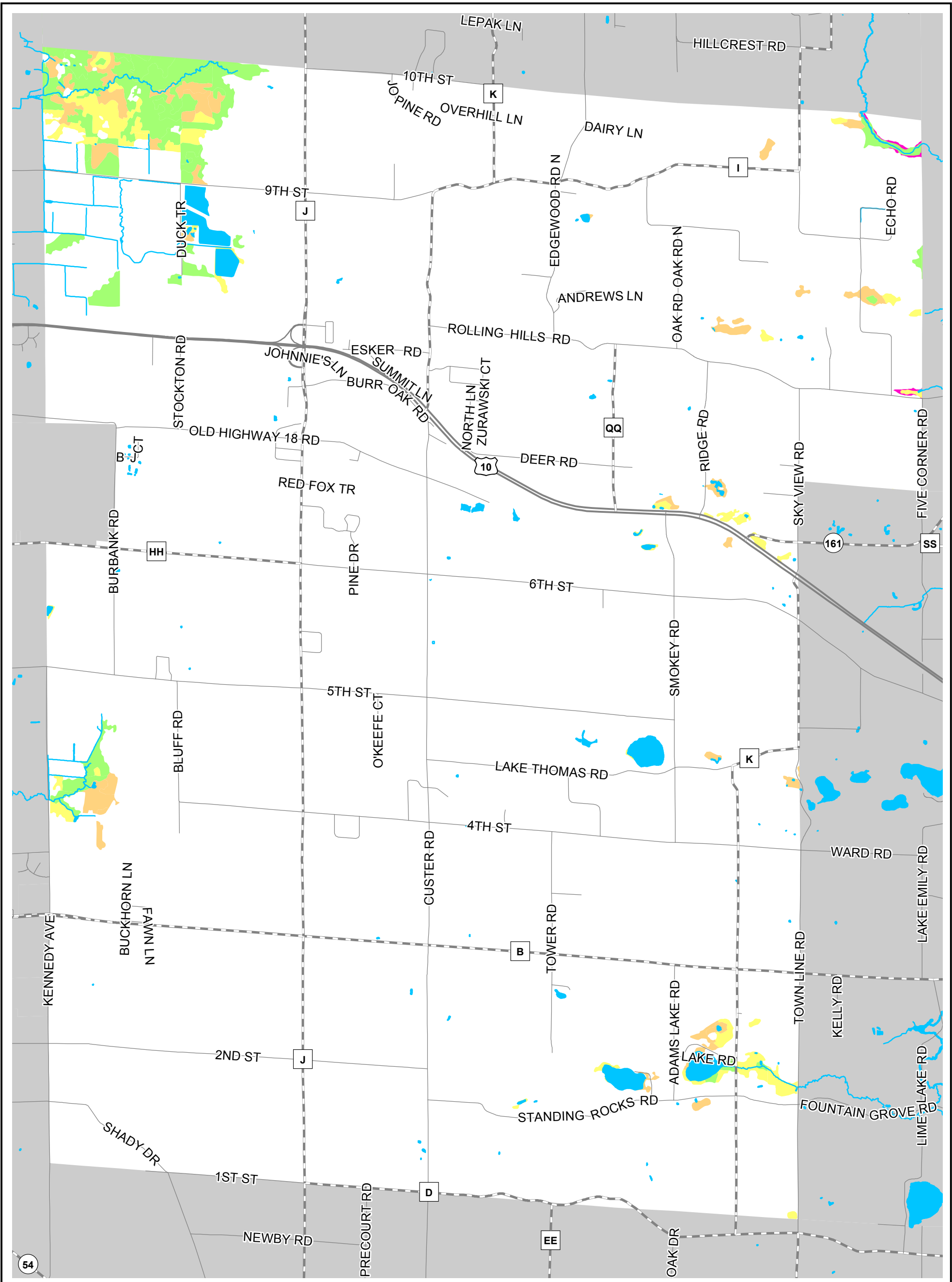
Map 5.4 Wetlands & Floodplain
