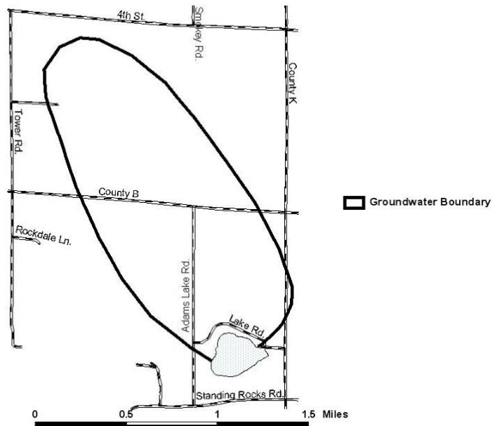
Adams Lake groundwater watershed boundary.
