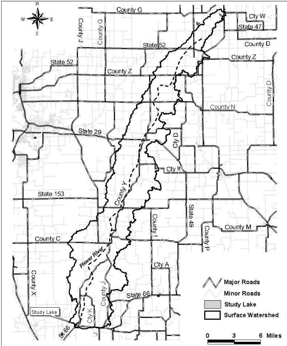
Jordan Pond surface watershed boundary.
