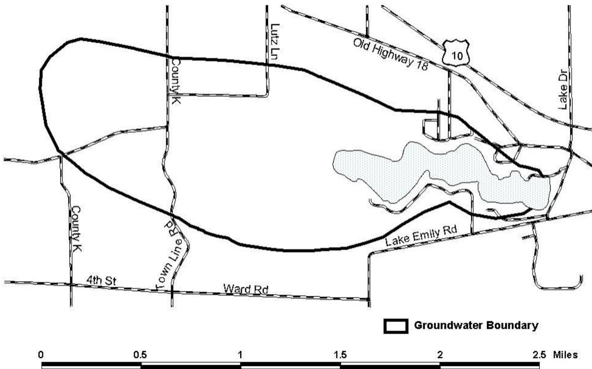
Lake Emily groundwater watershed boundary.
