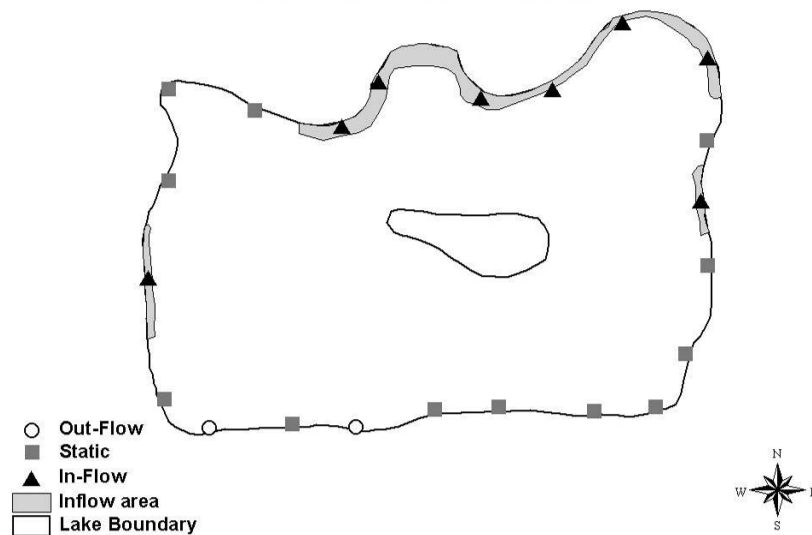
Figure 12. Locations in Joanis Lake showing groundwater inflow/no flow/outflow from mini-piezometer measurements and winter observations.
