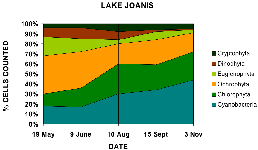
Figure 13. Algal community composition by date in Lake Joanis from May to November 2003 (total phylum cells counted divided by total cells counted).
