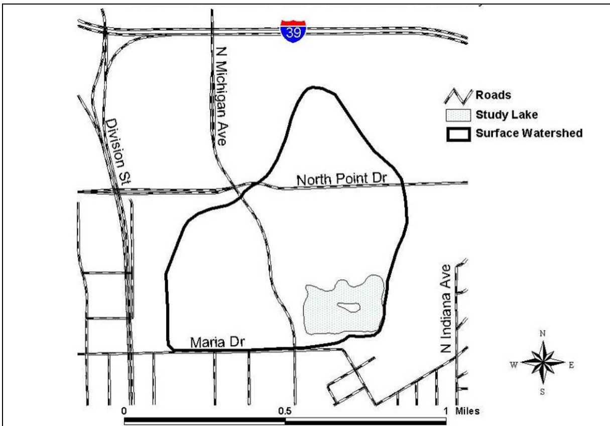
Figure 1. Lake Joanis surface watershed boundary.
