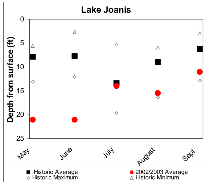
Figure 11. Monthly average water clarity measurements in Lake Joanis 2002-2003 and historic average, maximum and minimums.
