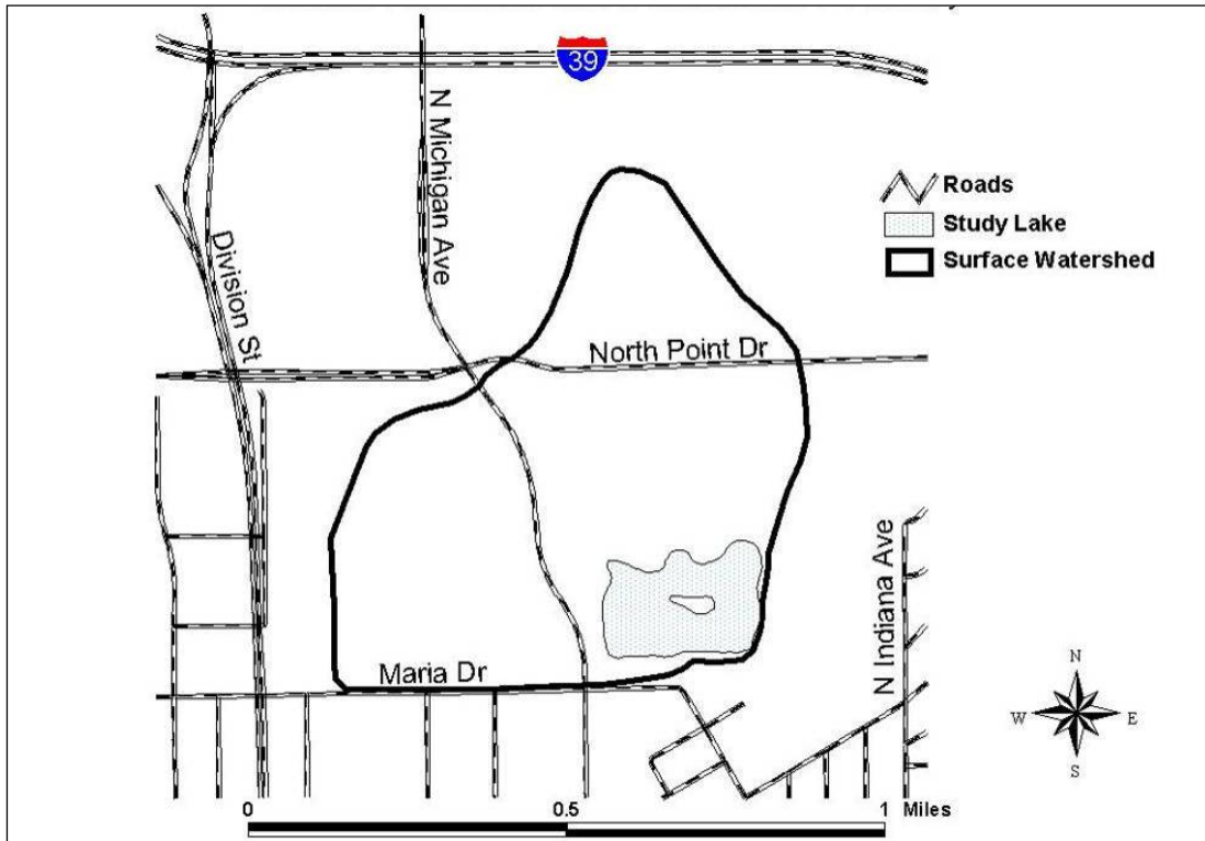
Lake Joanis surface watershed boundary.
