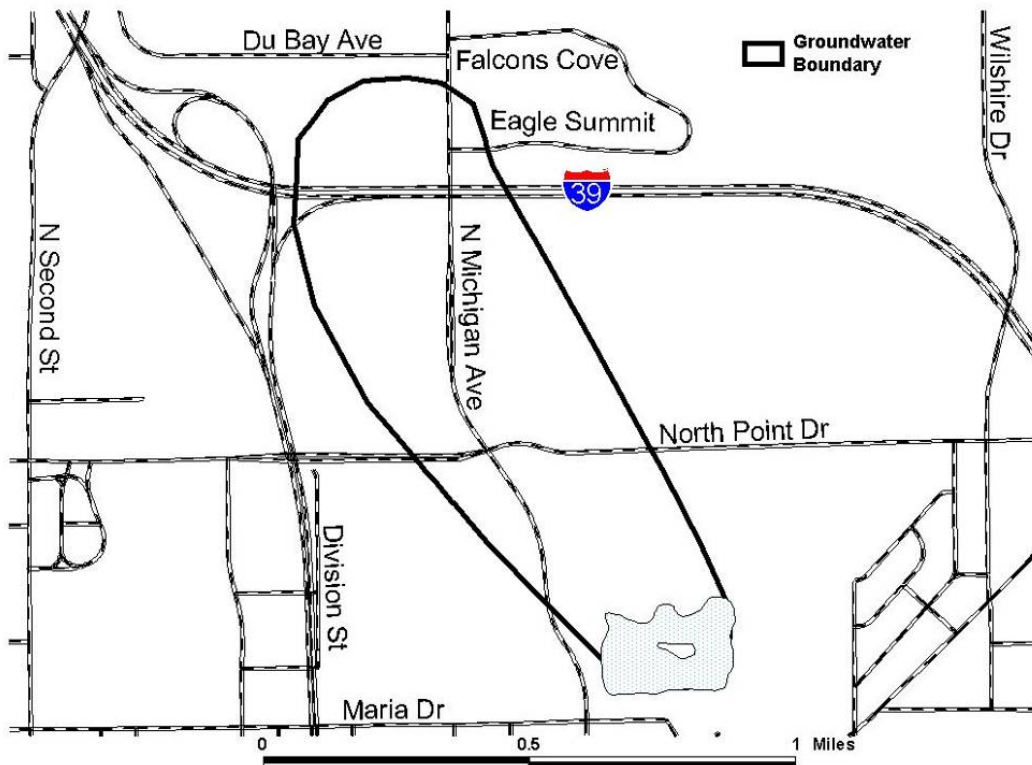
Lake Joanis groundwater watershed boundary.
