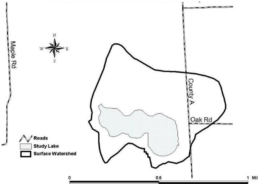
Lions Lake groundwater watershed boundary.
