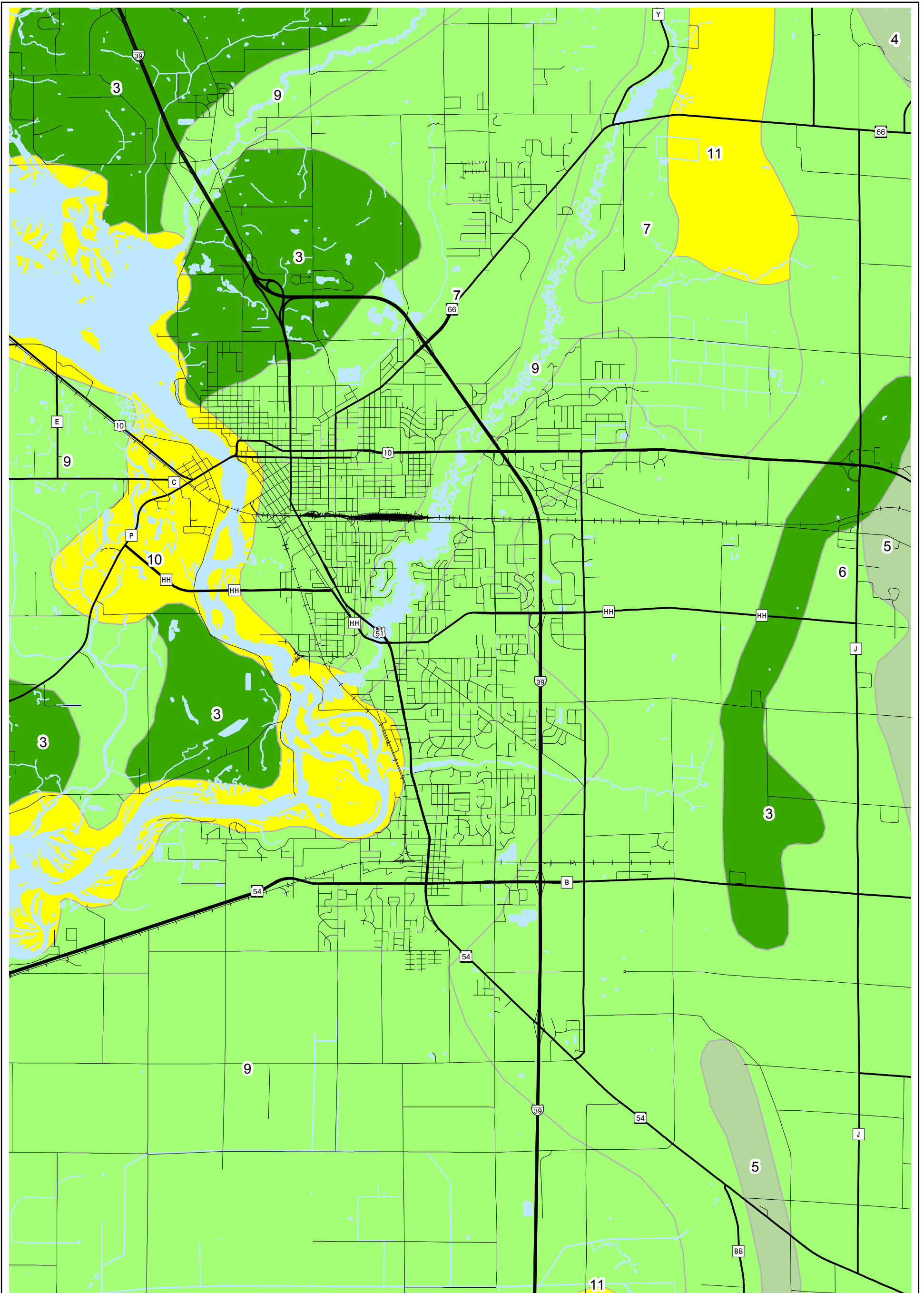
Map 2.2 General Soil Associations
